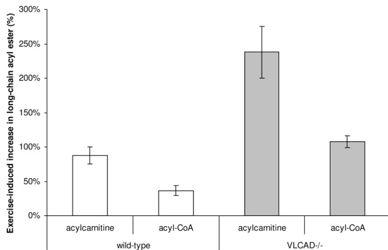
Fig. 3. Exercise-induced increase, as percentage of sedentary levels, in long-chain (C16:0, C18:2, and C18:1) CoA and carnitine esters in WT ( n = 4 ) and VLCAD -/- ( n = 5 ) mouse muscle. Values are means \pm SEM. Significances not tested. VLCAD, very long-chain acyl-CoA dehydrogenase; WT, wild type.
